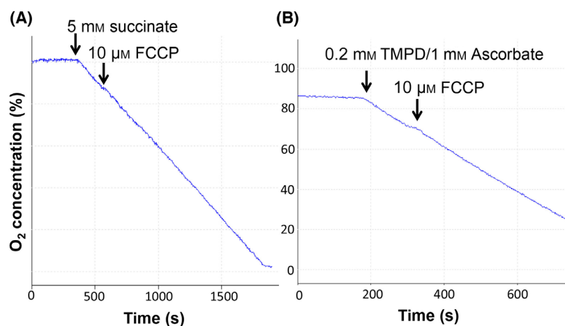
Fig. 4. FCCP has no direct inhibitory effect on the mitochondrial electron transport chain. (A, B) Isolated mouse liver mitochondria were subjected to a freeze–thaw cycle at -20^{\circ}\text{C} and then incubated in the Clarke electrode chamber in respiration buffer. The addition of 5 mM succinate and 10\ \mu\text{M} FCCP is indicated. (B) Intact isolated mouse liver mitochondria were incubated in respiration buffer, followed by the indicated additions of 0.2 mM TMPD ( N,N,N,N -tetramethyl- p -phenylenediamine) plus 1 mM ascorbate and 10\ \mu\text{M} FCCP.
